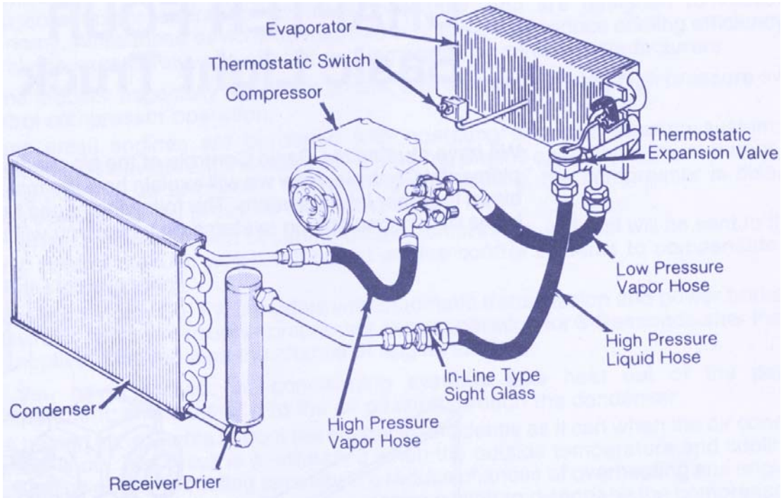
Expansion Valve Type System
