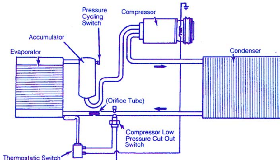
Accumulator Type Cycling Clutch A/C System
